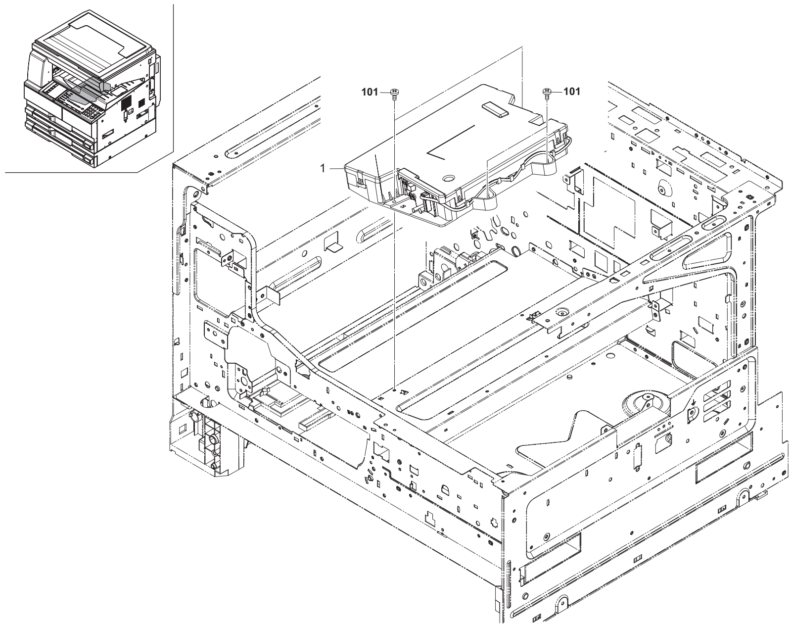
FIG. 12 Laser Scanner Section
