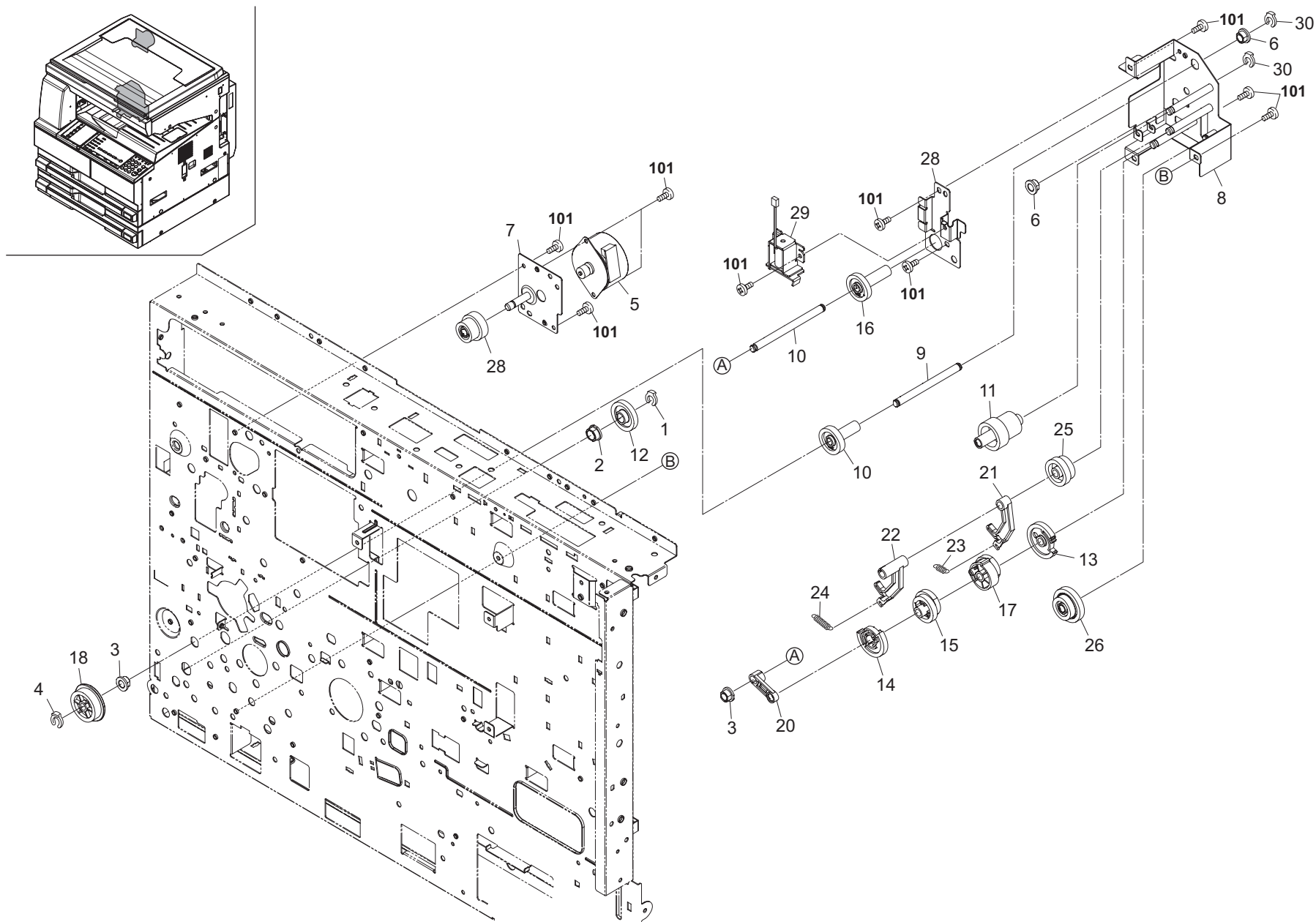
FIG. 16 Drive Section 1
