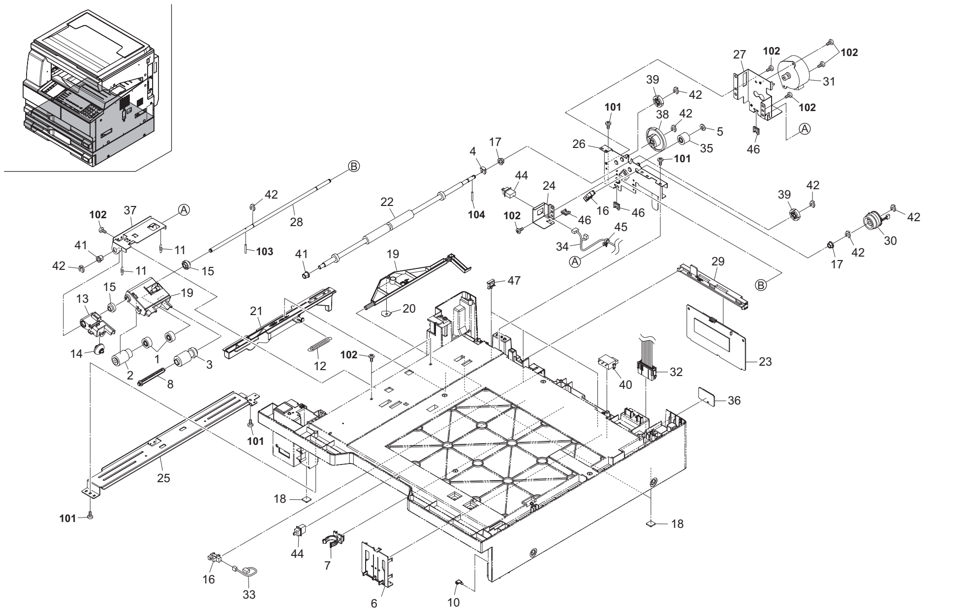
FIG. 7 Paper Feed Section 3 (22ppm)
