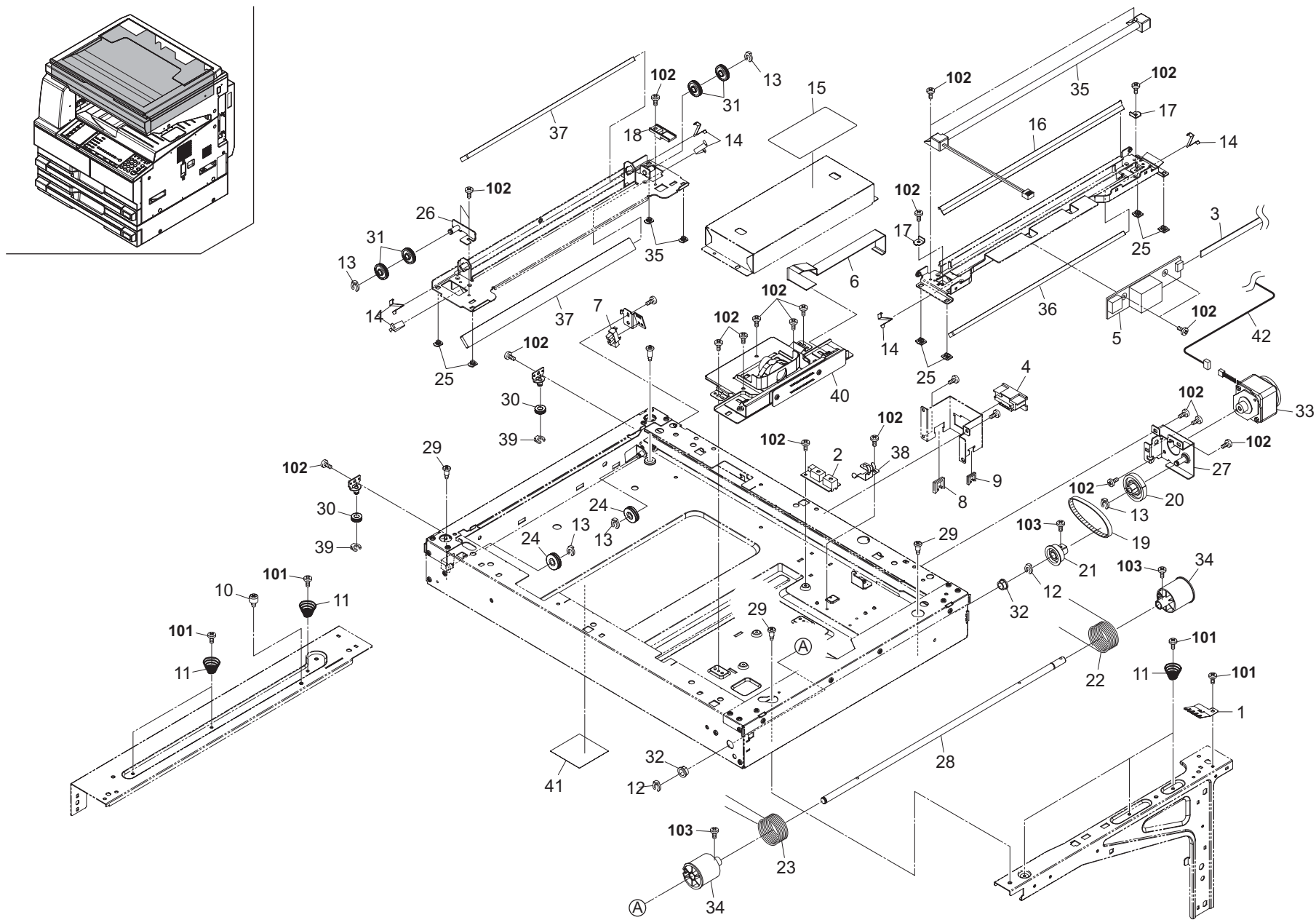
FIG. 10 Scanner Section 1
