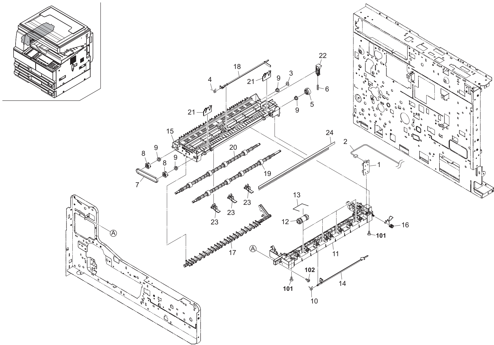
FIG. 18 Exit Section
