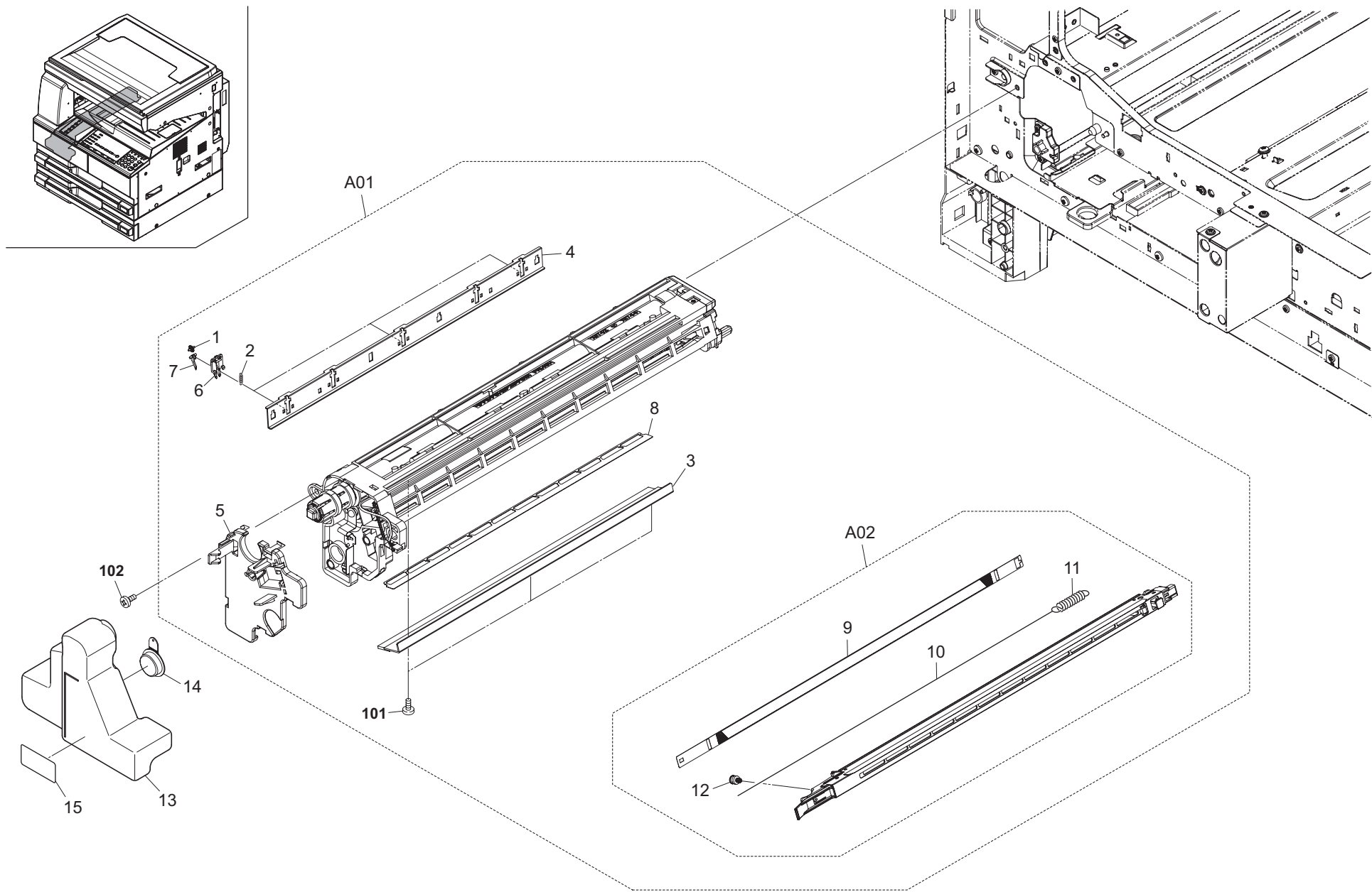
FIG. 13 Image Formation Section
