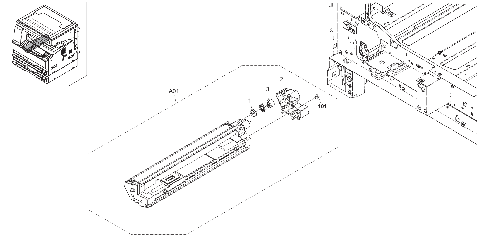
FIG. 14 Developing Section
