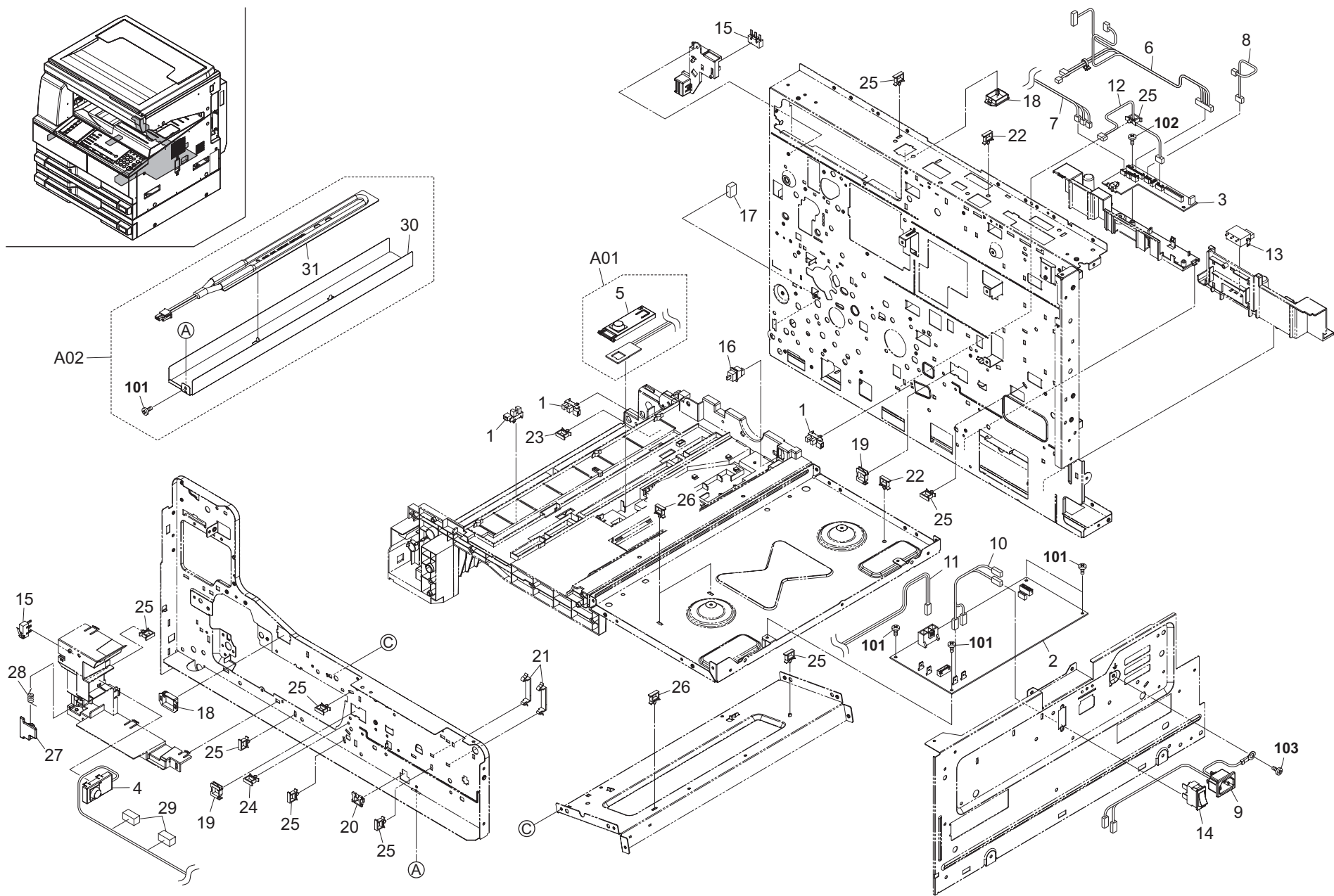
FIG. 19 Electrical Components 1
