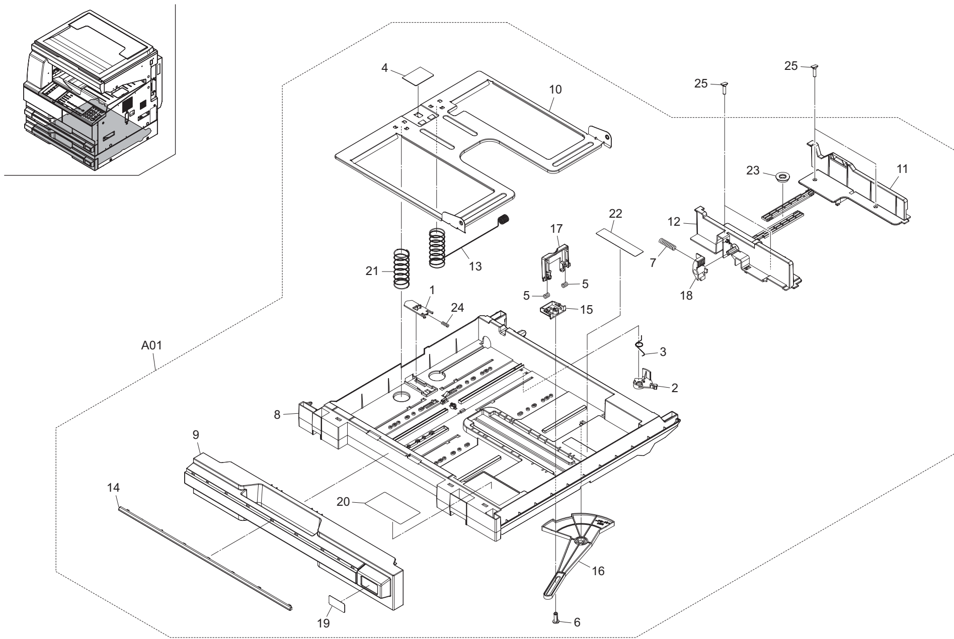
FIG. 9 Paper Cassette 2 (22ppm)
