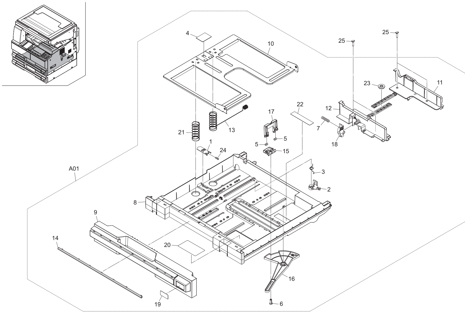
FIG. 6 Paper Cassette 1
