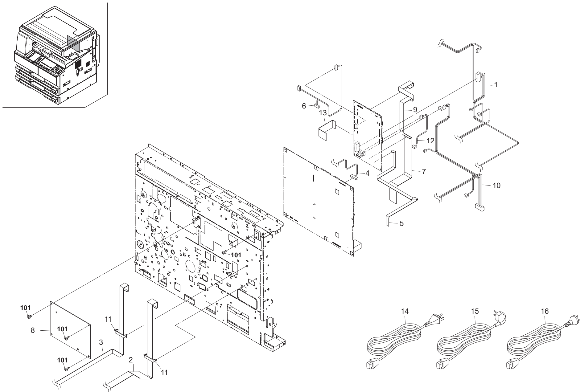
FIG. 20 Electrical Components 2
