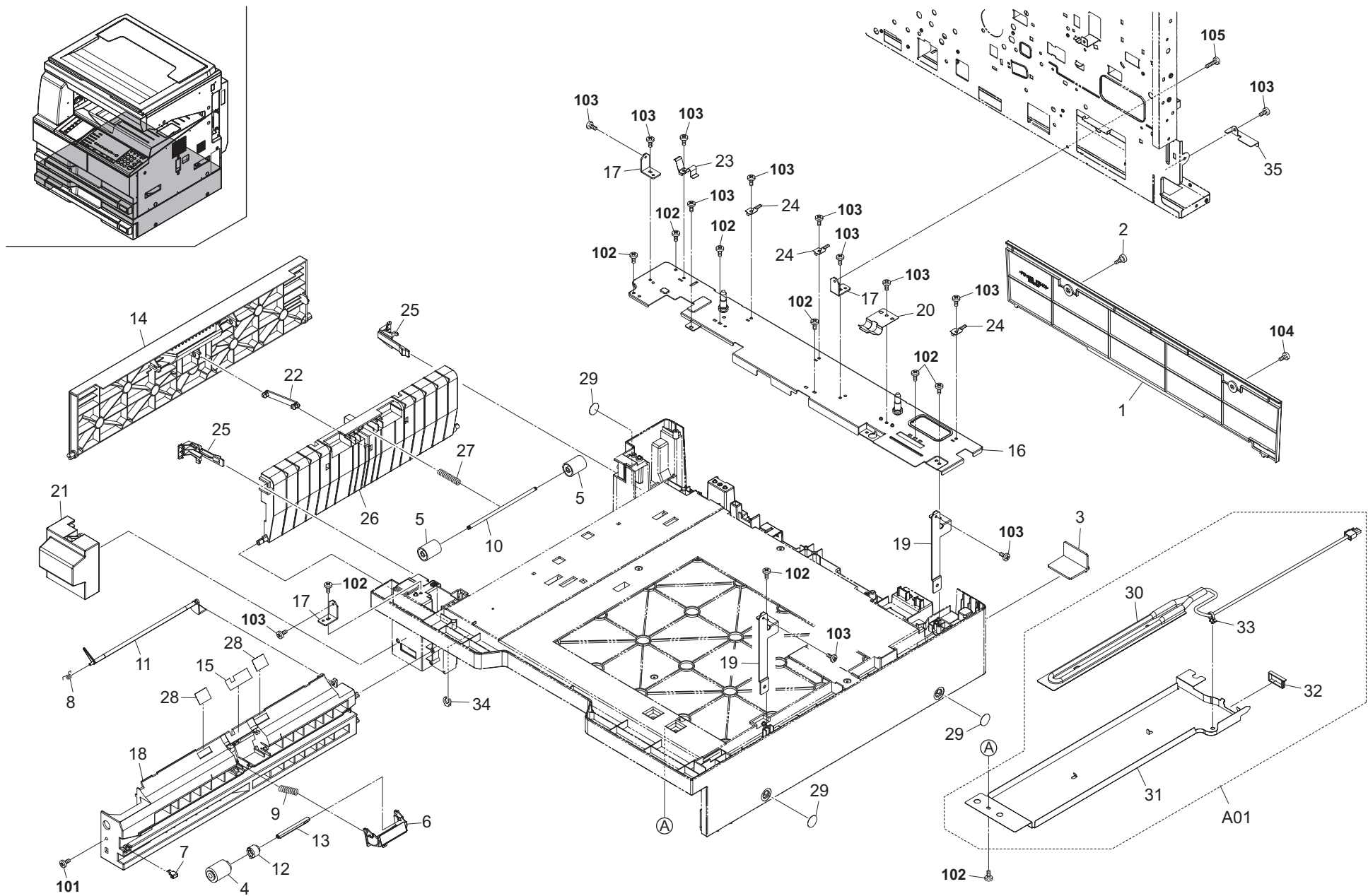
FIG. 8 Paper Feed Section 4 (22ppm)
