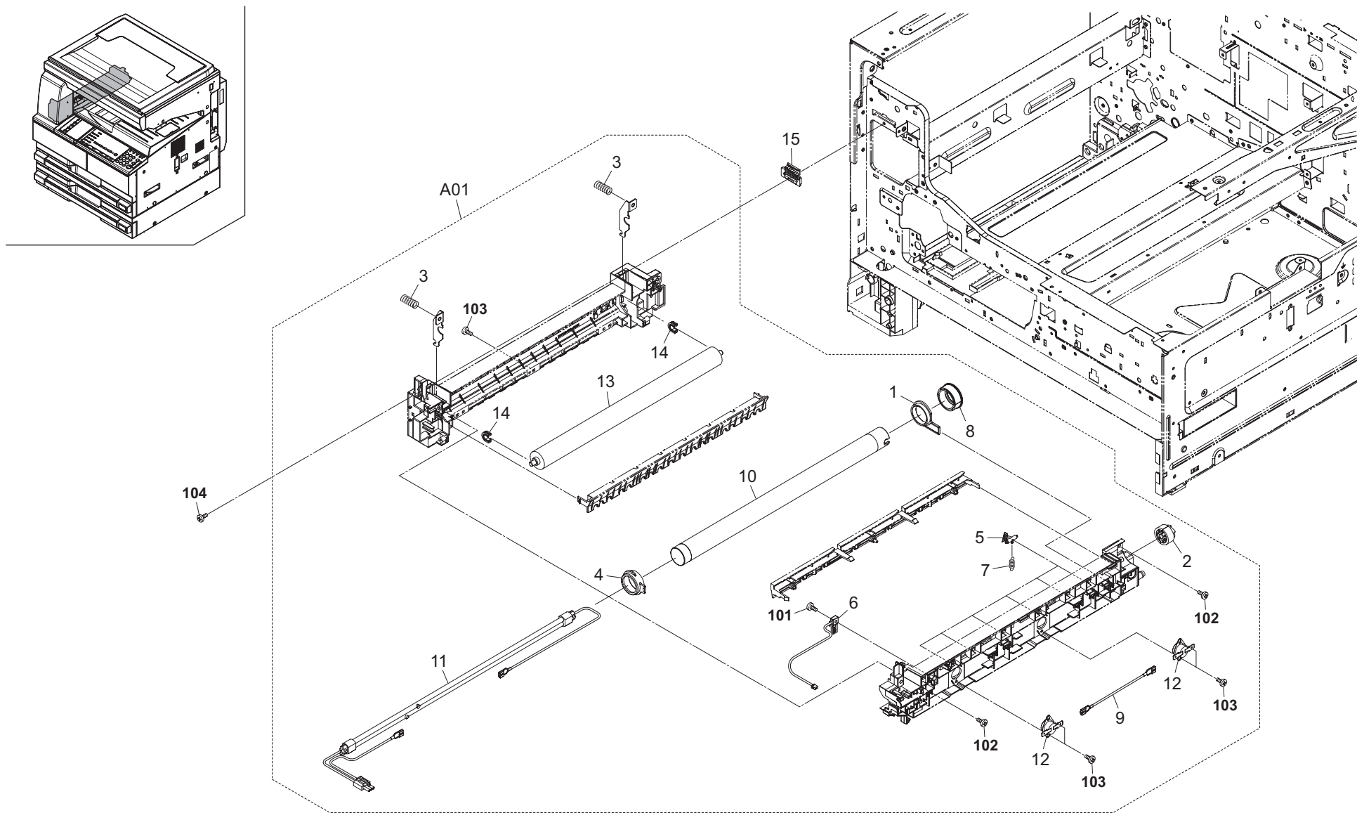
FIG. 15 Fuser Section
