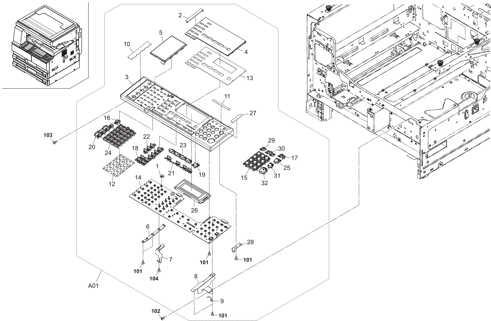
FIG. 22 Operation Section
