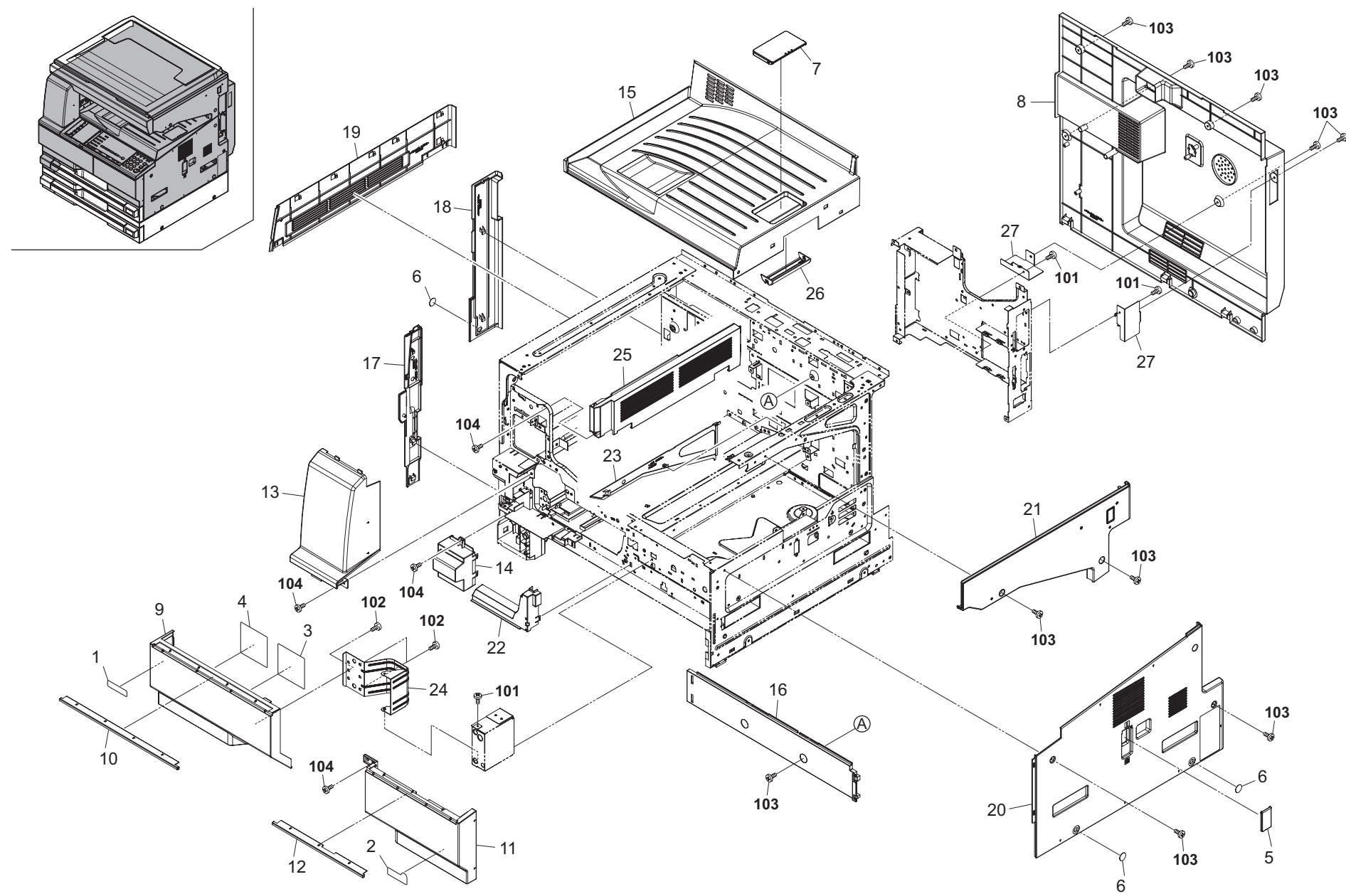
FIG. 1 Covers
